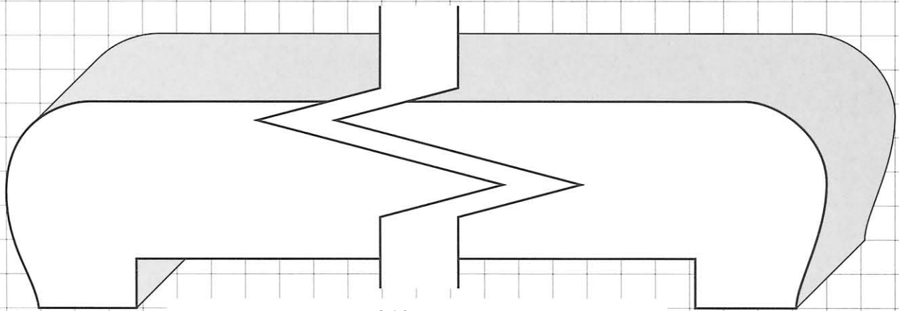
EC 840 Wall Cap 1 1 / 2 " Thick x Random Width (Specify Width of Check)
